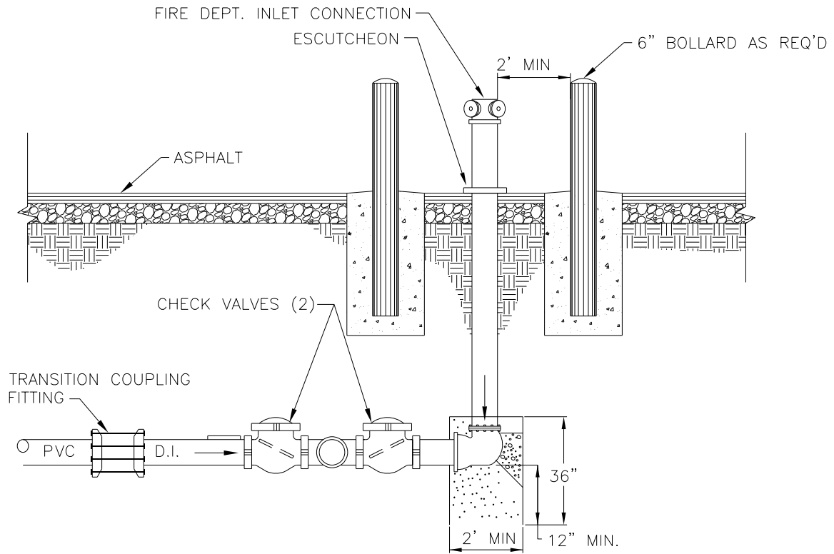
SECTION VIEW
