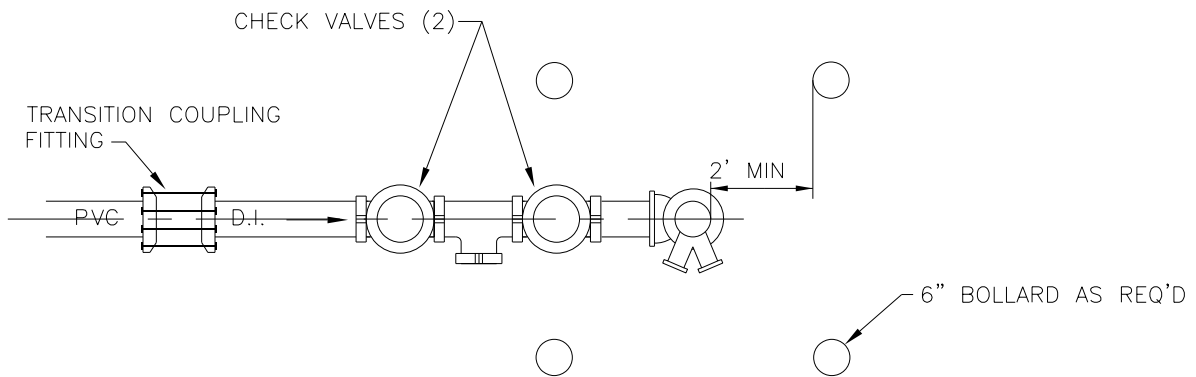
PLAN VIEW
