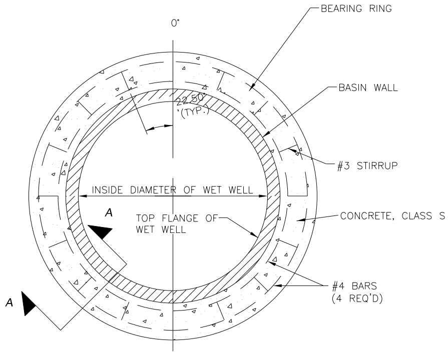
BEARING RING PLAN VIEW
