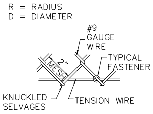
FABRIC & TENSION WIRE DETAIL TOP & BOTTOM
