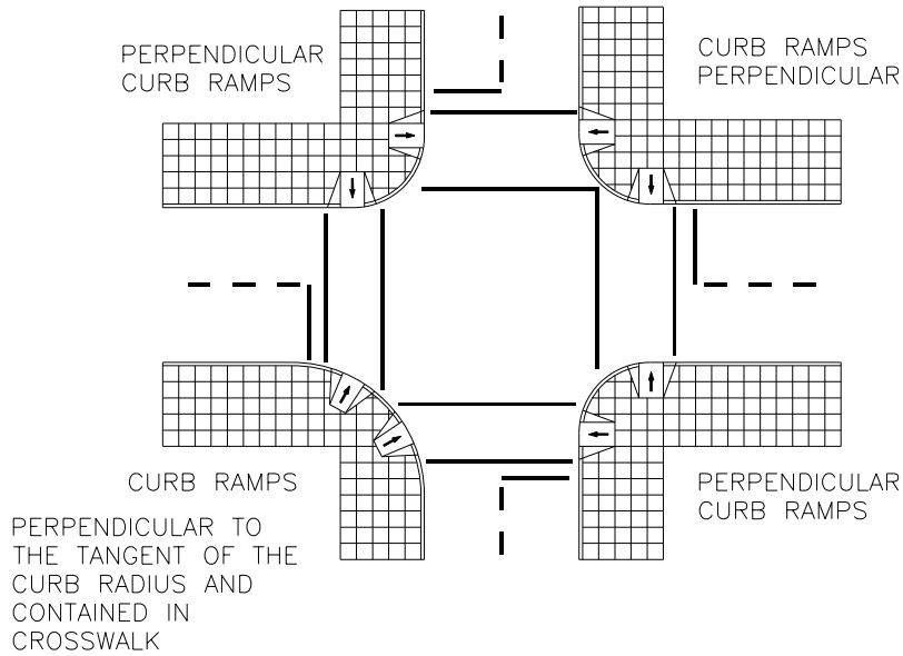
TYPICAL CURB RAMP PLACEMENTS AT INTERSECTIONS
