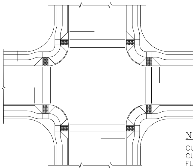
TYPICAL CURB RAMP PLACEMENTS AT INTERSECTIONS
