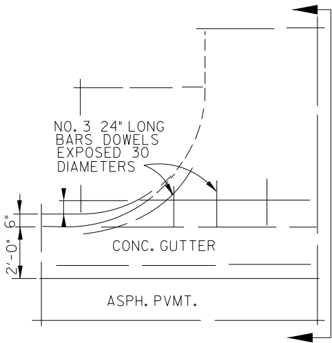
HALF PLAN ASPH. CONC. PVMT. WITH SEPARATE CONC. CURB AND GUTTER
