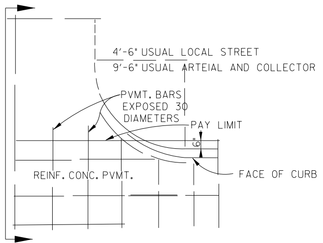
HALF PLAN REINF. CONC. PVMT. WITH INTEGRAL CONC. CURB
