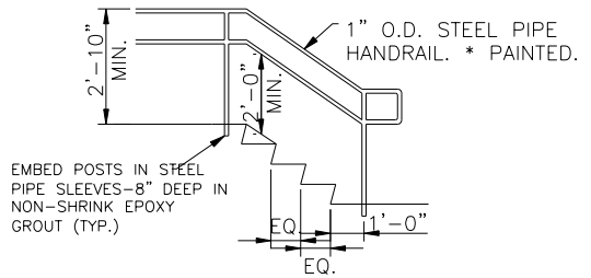
STAIR HANDRAIL
