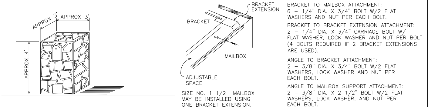
MAILBOX – MASONRY TYPE
