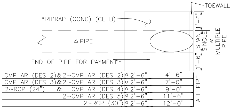
TYPICAL SECTION
