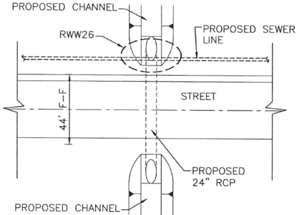
Figure 2a Typical Plan Sheet with Callout for Revised Detail
