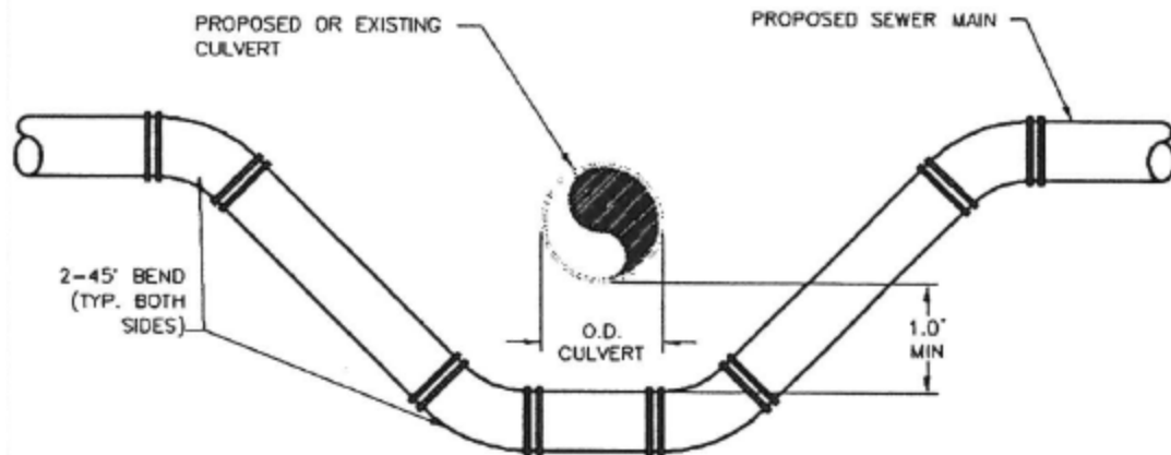
Figure 1b Standard Detail (from this Manual)
