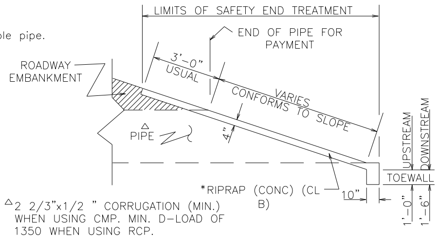
TYPICAL SECTION AT PIPE END
