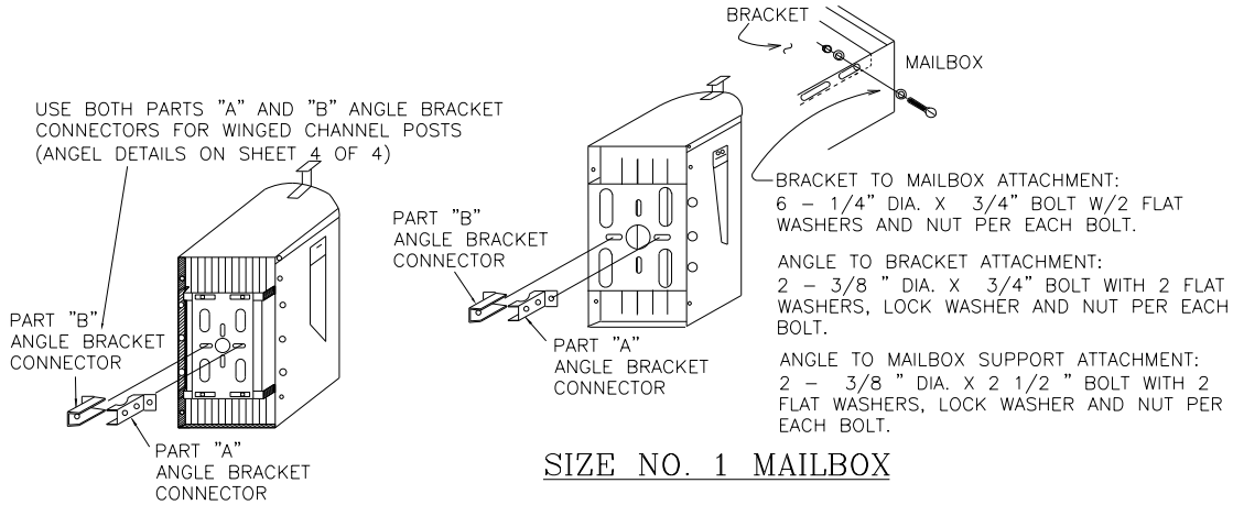
SINGLE MAILBOX – STANDARD MOUNT
