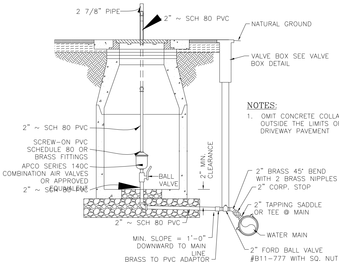
SECTION "Y-Y"
