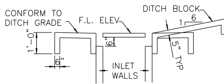
SECTION C-C RIPRAP DETAILS
