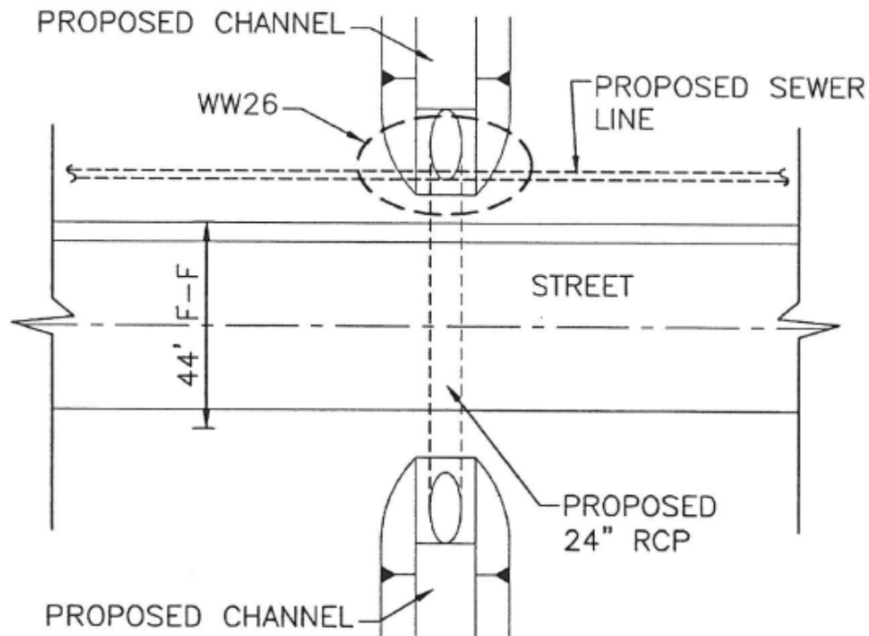
Figure 1a Typical Plan Sheet with Callout for Standard Detail
