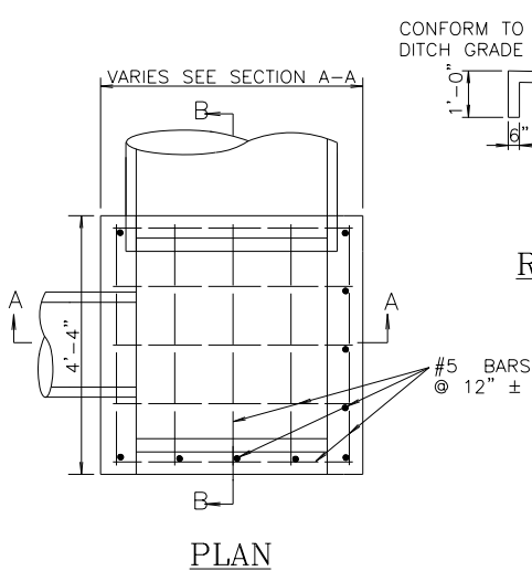
DITCH BLOCK PLAN
