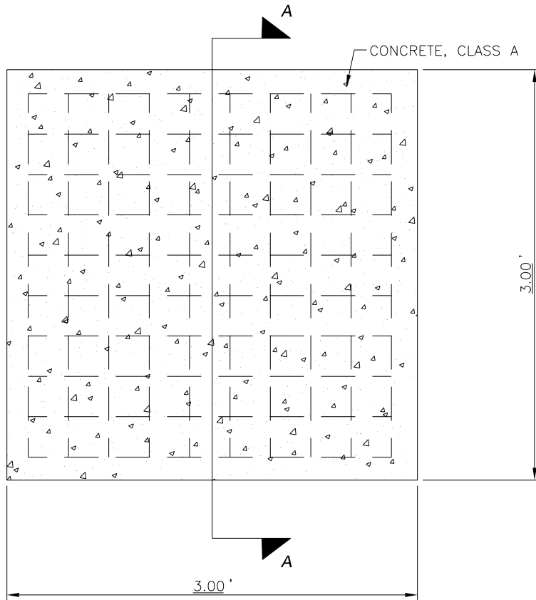
ODOR CONTROL SLAB PLAN VIEW N.T.S.
