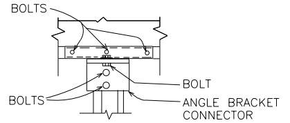
DETAIL A SINGLE MAILBOX MOUNT
