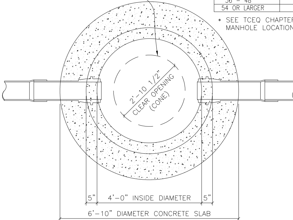
MANHOLE PLAN
