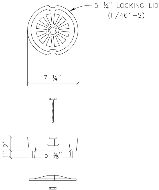
5 1/4" LOCKING LID (F/461-S)
