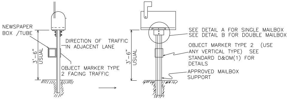
SINGLE MAILBOX – STANDARD MOUNT
