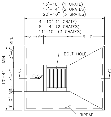
DITCH BLOCK PLAN
