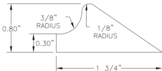
WEDGE TYPE GASKET TYPICAL DIMENSIONS
